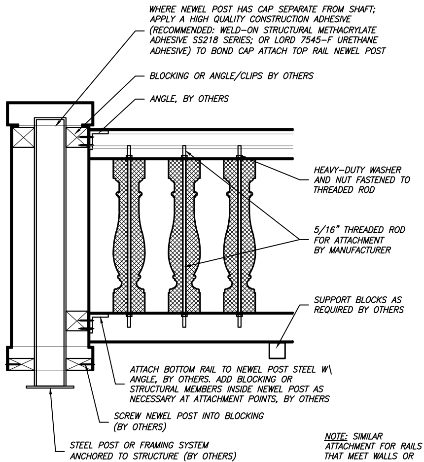
RAIL INSTALLATION - OPTION 1
