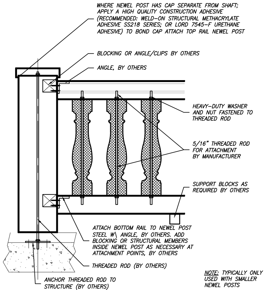
ALTERNATE NEWEL POST CONNECTION (DECORATIVE / NON-STRUCTURAL)
