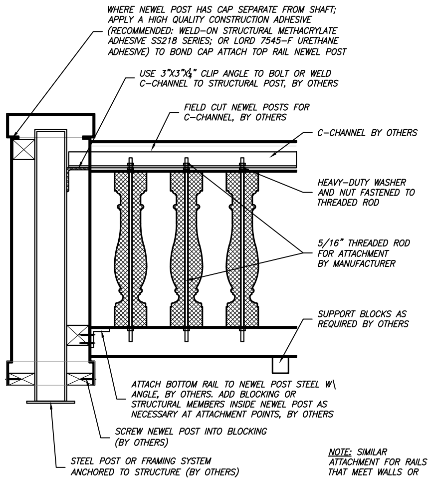
RAIL INSTALLATION - OPTION 2 (WITH C-CHANNEL)
